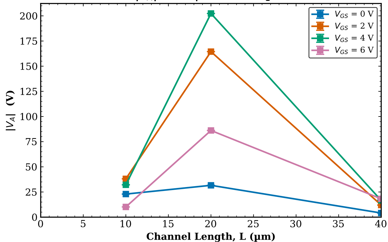
TFT3 Transistor 1 |V_A| vs L | W = 100\text{ }\mu\text{m}
